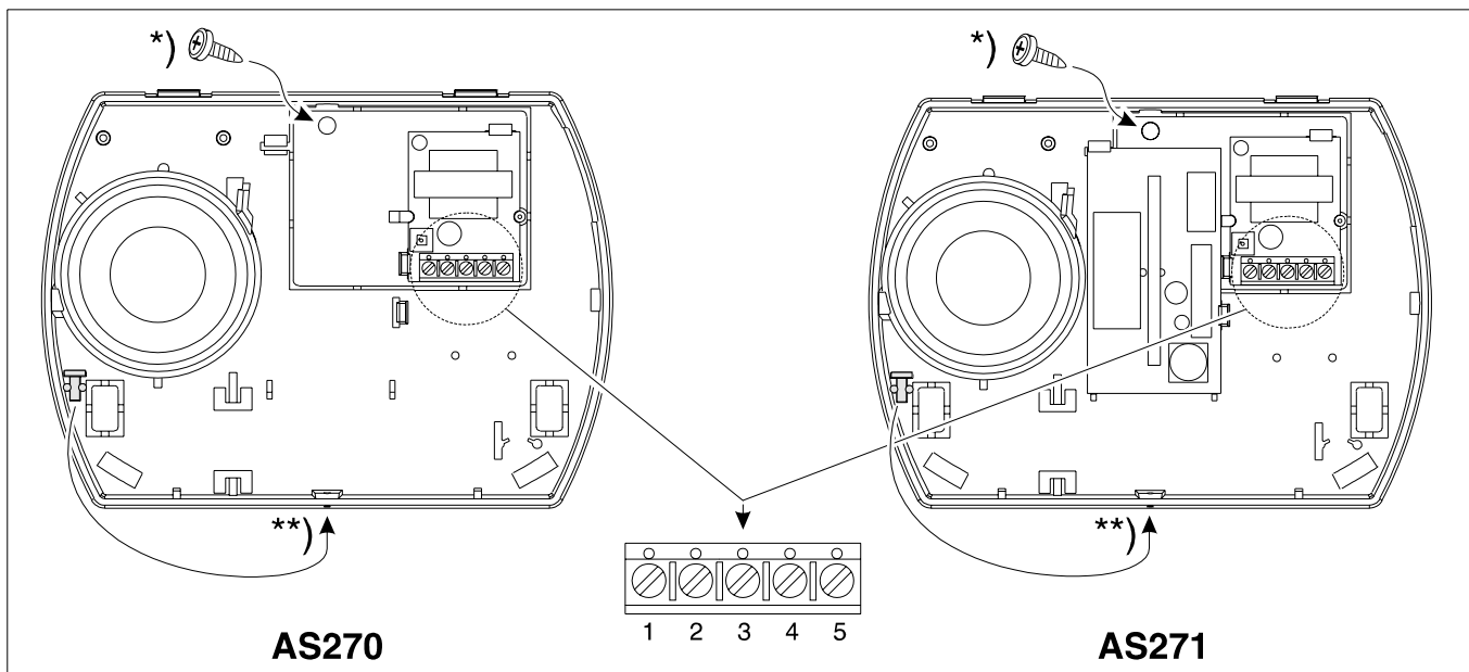
Abbildung 3: Innensirene AS 270/271
